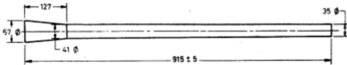
Fig. 2 Wooden Handle for Axes, Felling, Trade Pattern
